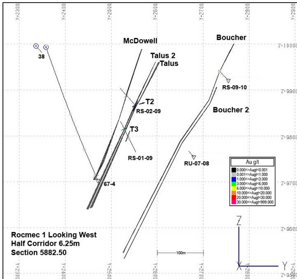
Figure 11: Section 5882.5mE
