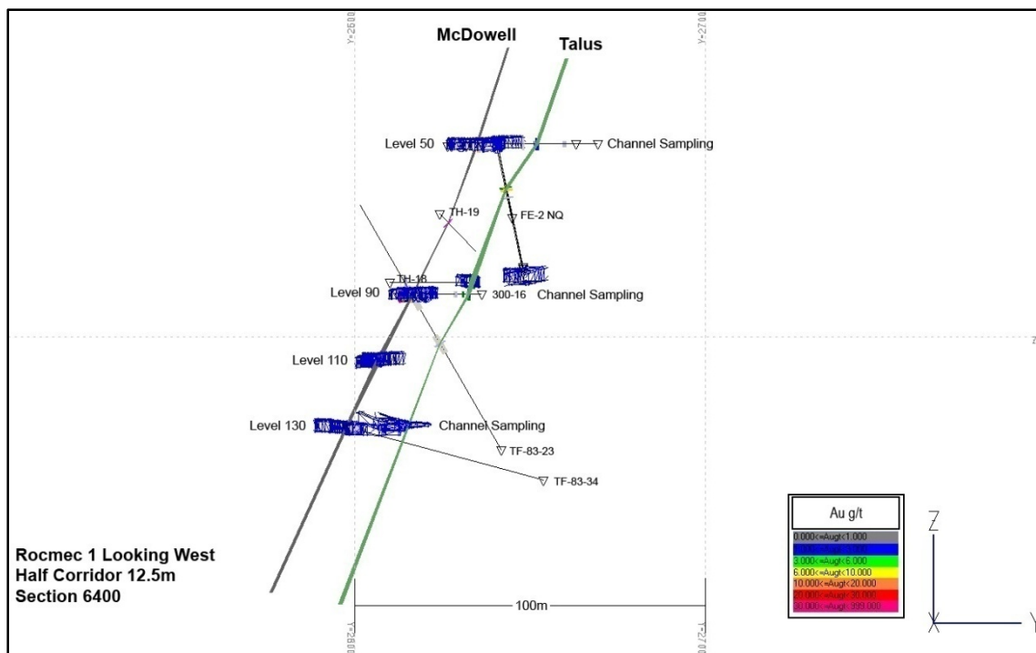
Figure 16: Section 6400mE
