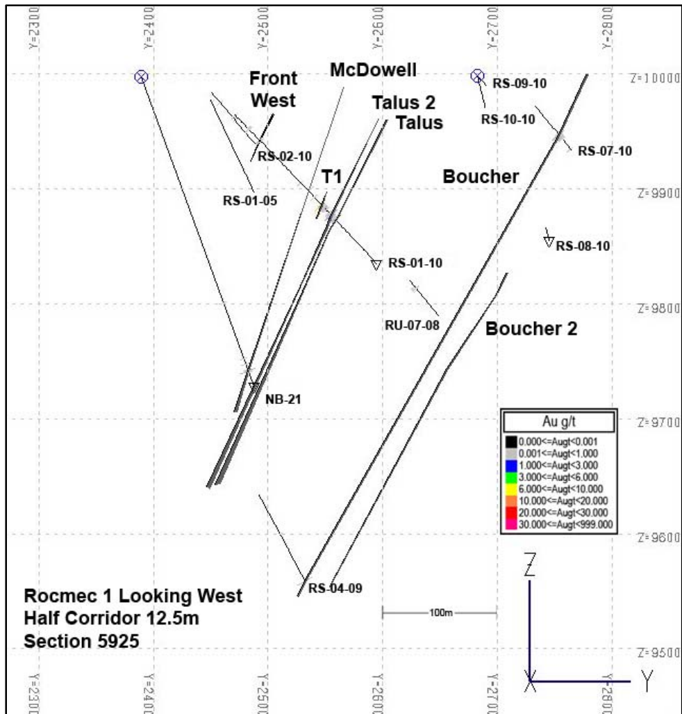
Figure 12: Section 5925mE
