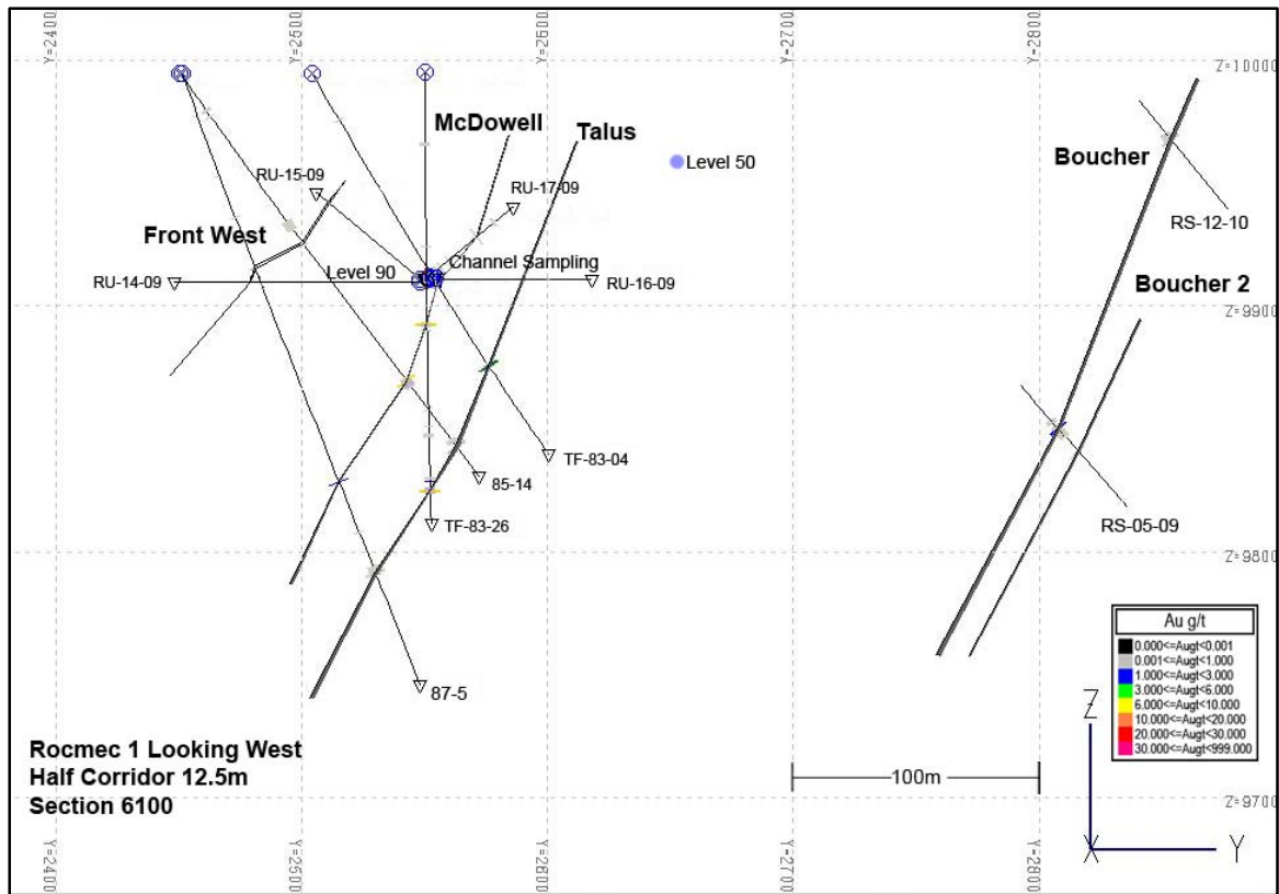
Figure 15: Section 6100m
