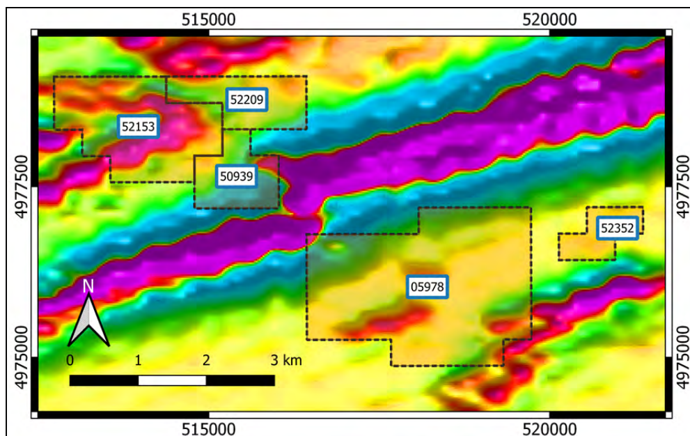
Figure 9-1 - Aeromagnetic Map, 2nd Vertical Derivative, NSDNR, 1997
