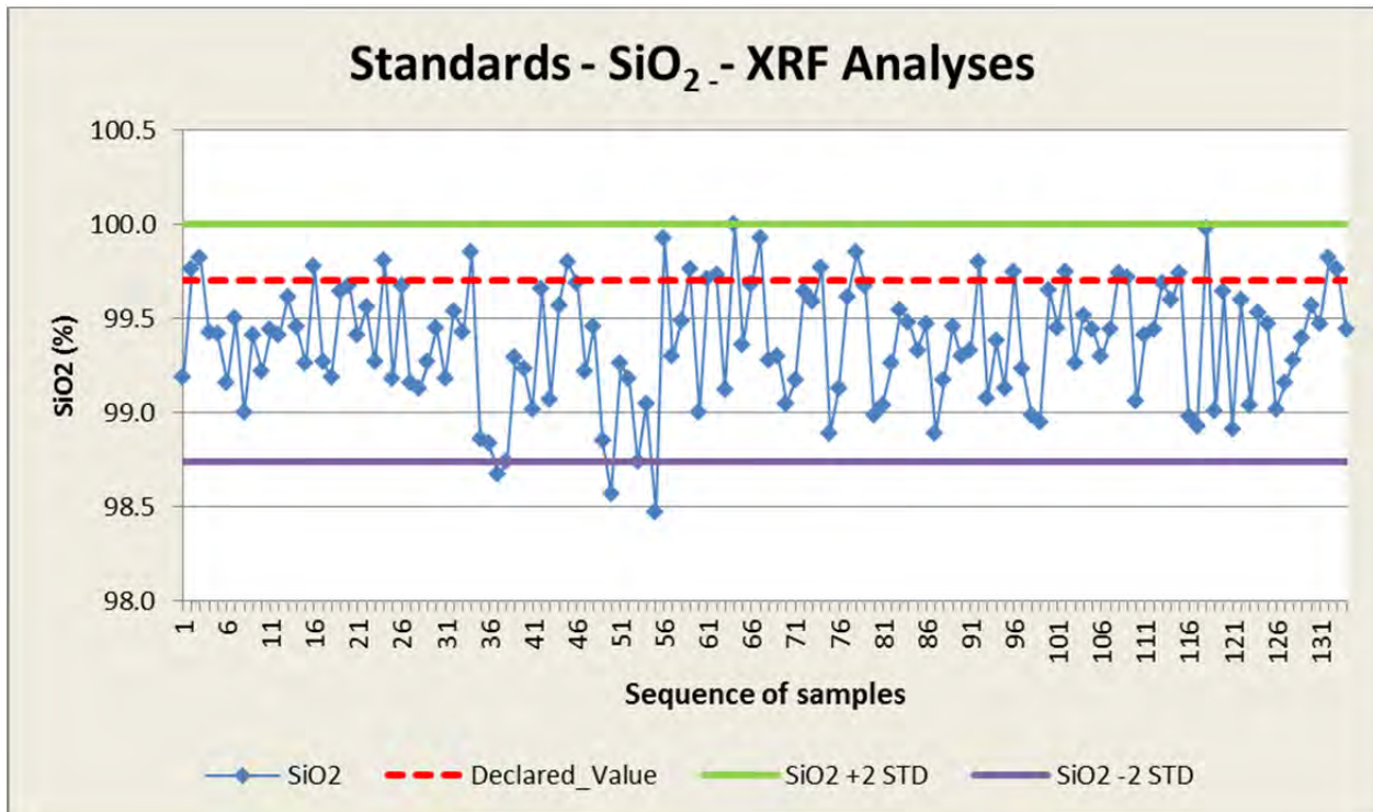
Figure 12-10: Analysis of Silica by XRF for the Reference Material
